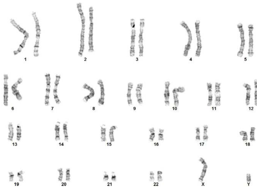
Figure 5. G-banding karyogram
