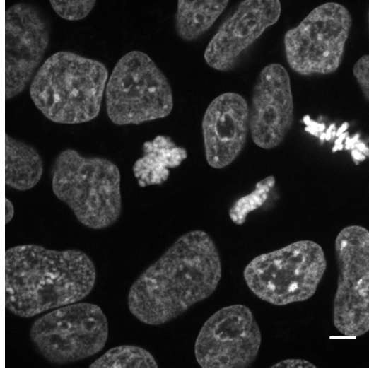
Figure 3: Single, mid-level plane of cells in a live hiPS cell colony expressing mEGFP-tagged Histone H2B type 1-J protein. The cells in the imaged region highlight cell-cycle-dependent changes in localization. The large dim regions within nuclei likely represent nucleoli. Cells were imaged in 3D on a spinning-disk confocal microscope. Scale bar, 5 \mu\text{m} .
