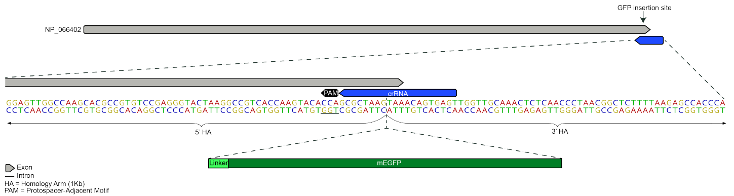
Figure 1: Top: HIST1H2BJ locus; Bottom: Zoom in on mEGFP insertion site at HIST1H2BJ C-terminus
